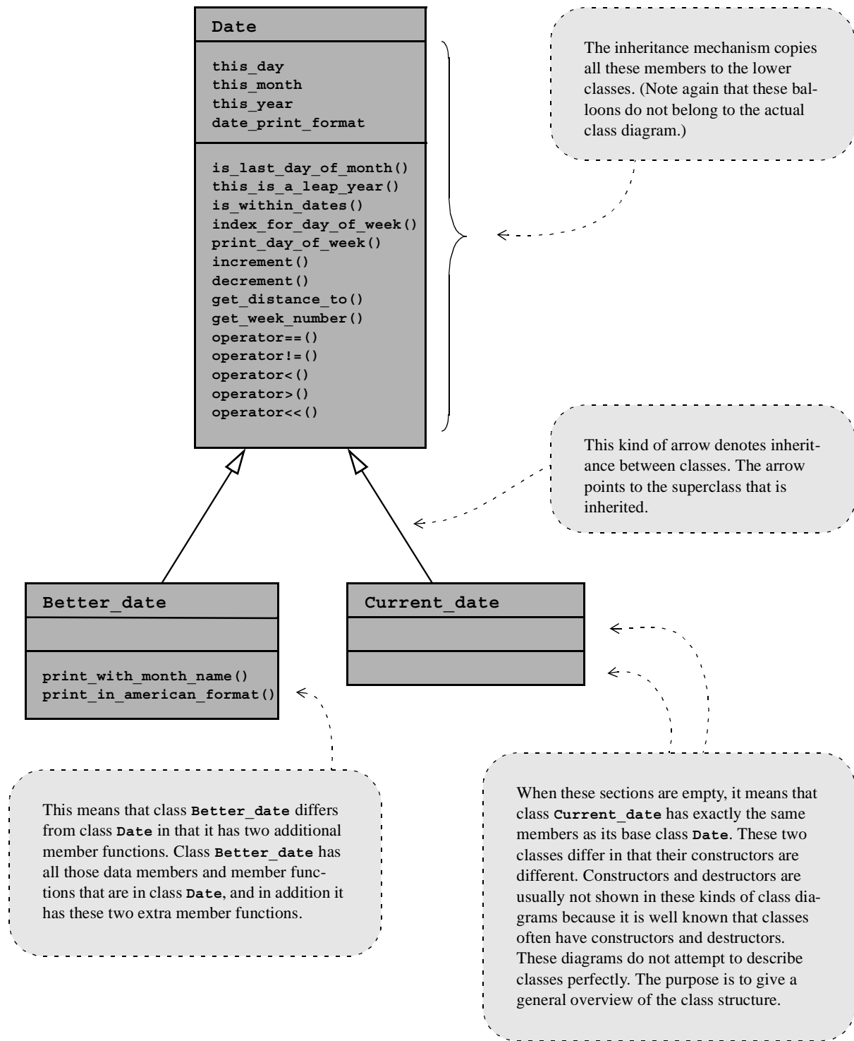
Figure 14-1. Class diagram that describes relationships between three classes.
